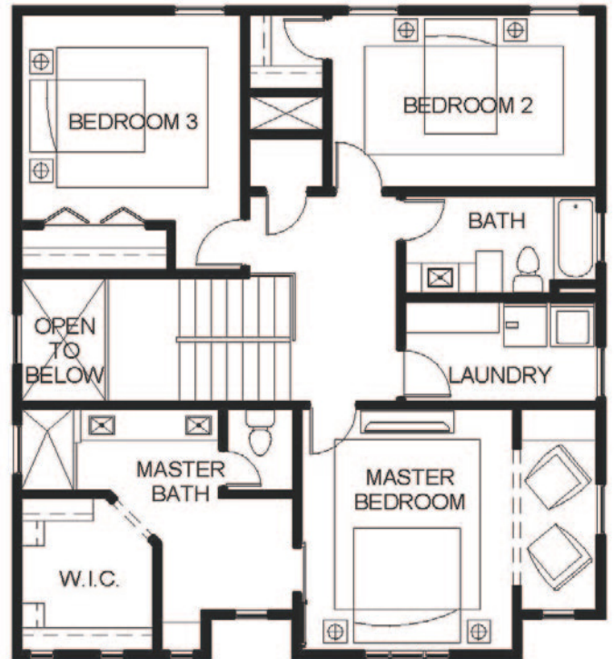
Upstairs Floorplan
